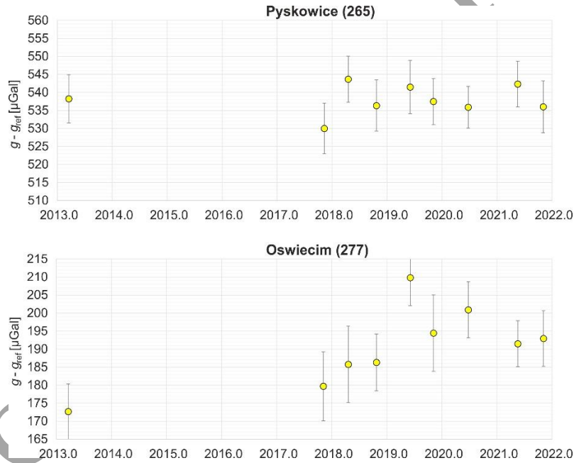
Fig. 2. Absolute gravity measurements conducted within the EPOS-PL project at PBOG stations in Pyskowice ( g_{\text{ref}} = 981\,069\,000 ; top) and Oswiecim ( g_{\text{ref}} = 981\,034\,000 ; bottom); error bars indicate the total uncertainty of gravity value determined with A10-020 gravimeter, reduced to benchmark level, single coverage k = 1 , 67%
