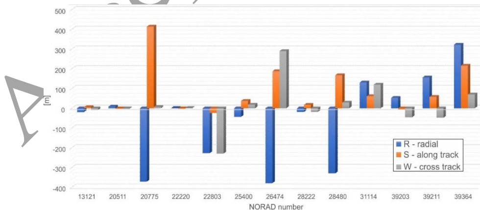
Fig. 3. Input TLE ephemerides vs. laser measurements in RSW frame
