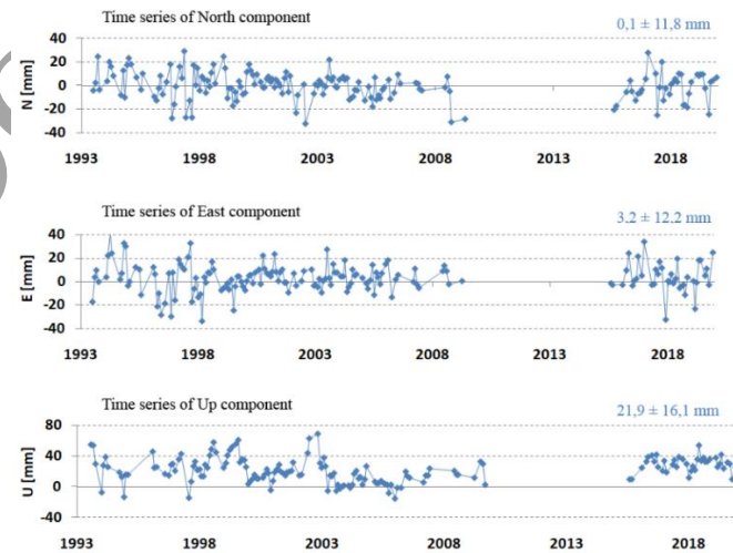
Fig. 5. De-trended for epoch 2010.0 topocentric coordinates N, E, U of BORL station in 1993-2019 ([63]Schillak et al., 2022)
