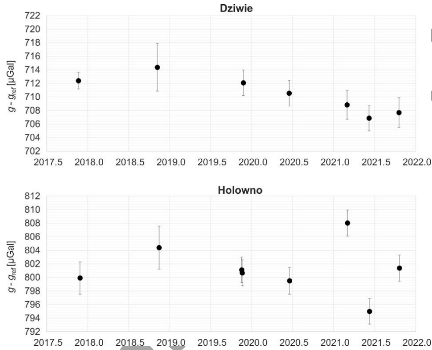
Fig. 3. Absolute gravity measurements within MGP project at stations in Dziwie ( g_{\text{ref}} = 981\,216\,000 ; top) and Holowno ( g_{\text{ref}} = 981\,115\,000 ; bottom); error bars indicate the total uncertainty of gravity determined by the FG5-230 gravimeter at 125.0 cm height above benchmark level, single coverage k = 1.67\%
