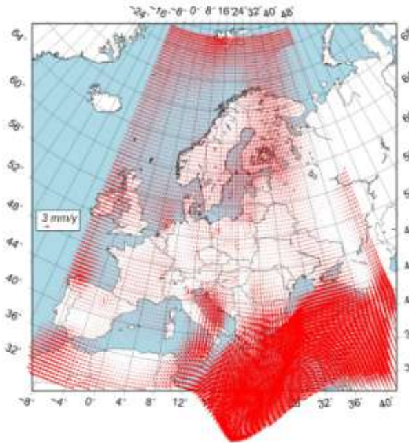
Fig. 9. The continuous intraplate velocity field for Europe with the use of APKIM2005 (IGN) model
