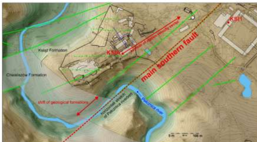
Fig. 17. Location of the new established GPS station KSI1 in relations to the existing station KSIA.
