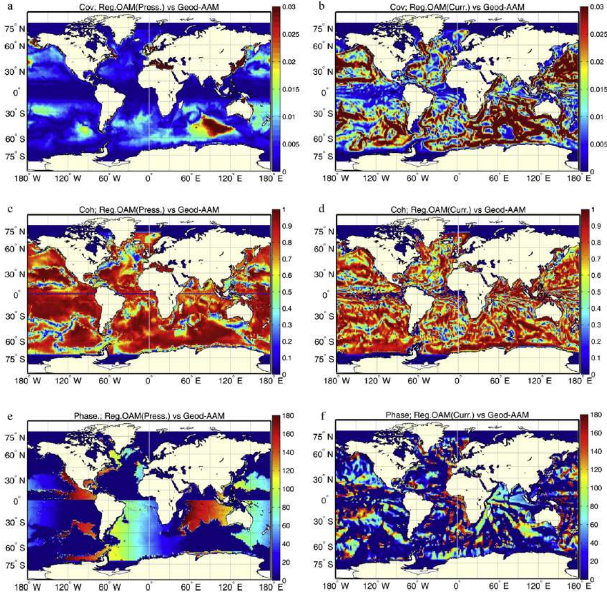
Fig. 5. Maps of (a, b) magnitude of covariances, (c, d) magnitude of coherence (e, f) and phase between prograde components of signals in the band around the Chandler oscillation of regional OAM (left panels pressure, right panels currents) and of global non-atmospheric geodetic excitation function (Nastula et al., 2012)
