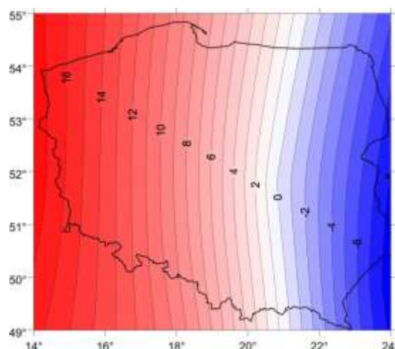
Fig. 24. Time shift between the records of the stations and others European observatories and Belsk Observatory records ( Y component) (Welker, 2011)
