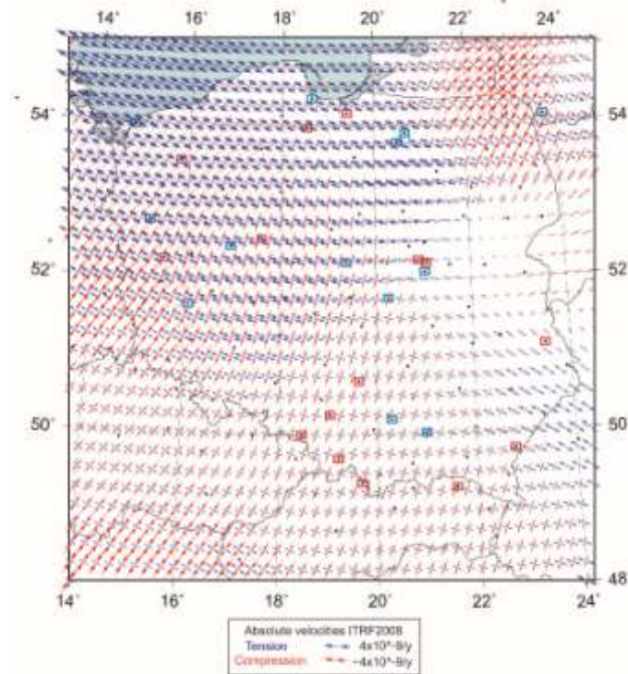
Fig. 11. Continuous strain field after the final data verification (the excluded stations are also marked to show what influence they had on the appearance of the strain field) (Bogusz et al., 2013a)
