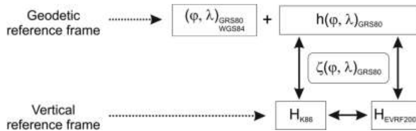
Fig. 14. The relationship between geodetic and vertical reference frame realizations of Polish National Spatial Reference System
