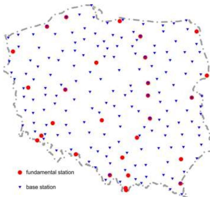
Fig. 18. Stations of new gravity control in Poland
