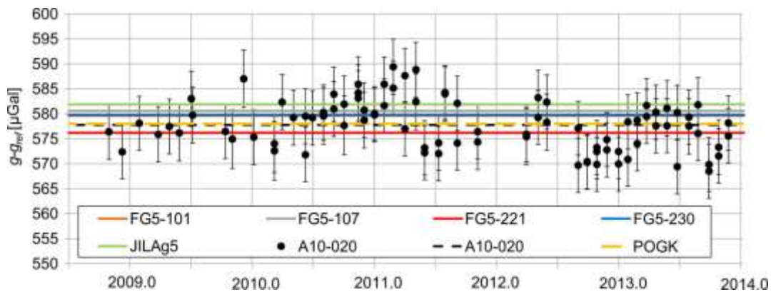
Fig. 11. Results of absolute gravity measurements with A10-020 at Borowa Gora
