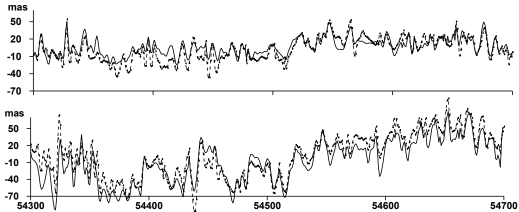
Fig. 2. An example of common oscillations in the equatorial components ( \psi_1/\chi_1 - upper graph, \psi_2/\chi_2 - lower graph) of geodetic (solid line) and fluid AAM+OAM+HAM (dashed line) excitation functions, computed using wavelet based semblance filtering with threshold value equal to 0.90 (Kosek et al., 2011a)
