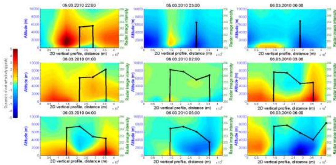
Fig. 7. Cross section of tomography model along the storm propagation line (from 0 to 10 000 m), colour-coded are wet refractivities variations in time, whereas the black line shows the radar rain intensity and location of storm
