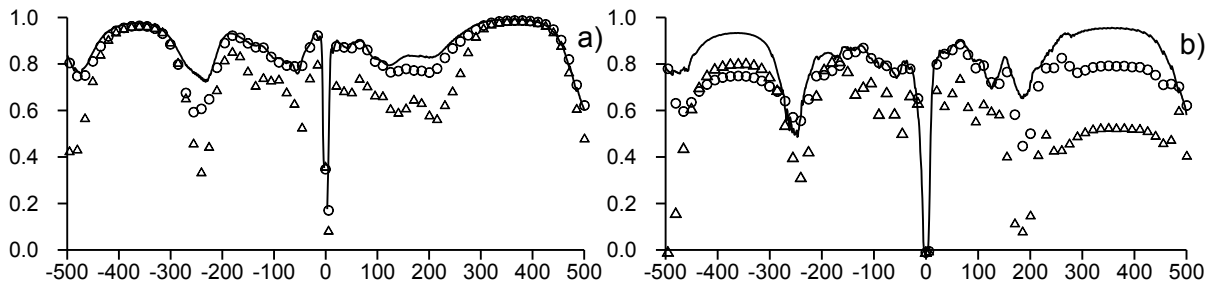
Fig. 1. The semblance functions of the orders 0 a) and 3 b) between the polar motion geodetic and fluid excitation functions AAM (triangles), AAM+OAM (circles) and AAM+OAM+HAM (solid line) (Kosek et al., 2011a)
