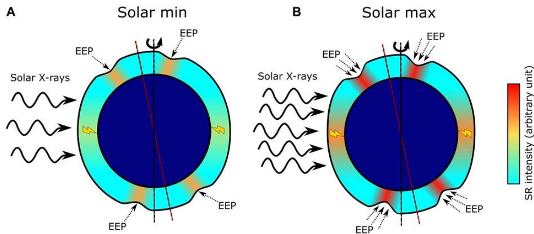
Figure 1. Illustration of the deformation of the Earth-ionosphere cavity at solar minimum (A) and solar maximum (B). At solar maximum X-rays and EEP reduce the cavity height more significantly (dominantly over low- and high latitudes, respectively) which results in enhanced SR intensity values beneath the deformed regions. Reprinted from Bozóki et al. (2021)
