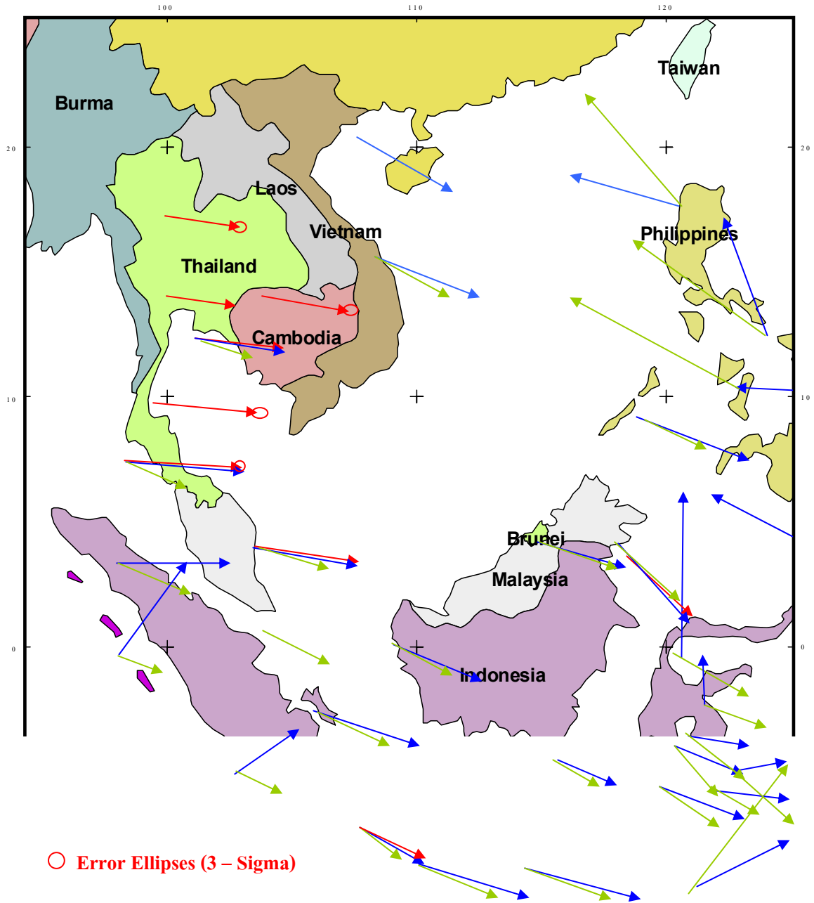
Fig. 7 Thailand 1994-2001 Horizontal Velocities in ITRF-2000
